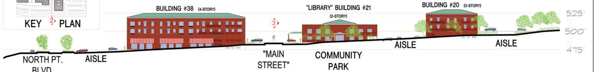
1 SS SITE SECTION @ CROSS STREET LOOKING NORTH
